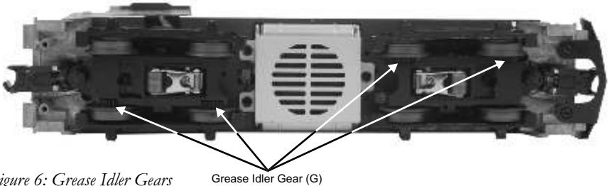
Figure 6: Grease Idler Gears
