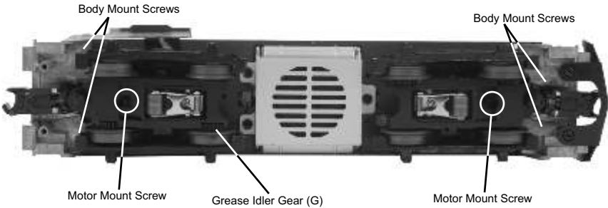
Figure 5: Body Removal Screw Locations and Motor Mounting Screws
