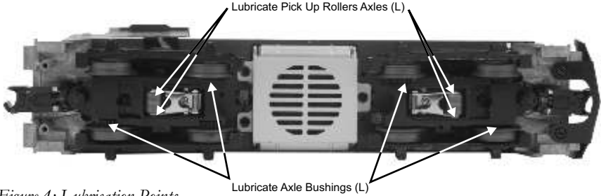
Figure 4: Lubrication Points
