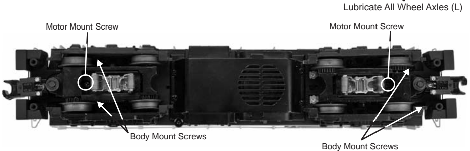
Figure 7: Body Mount Screws
